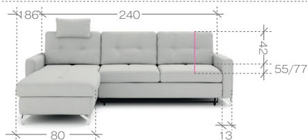
narożnik > corner sofa OSBL**+2FBP*(206x143) 1. paczka | package - OSBL - 188x85x80 cm (1,28m 3 , 55,5kg) 2. paczka | package - 2FBP - 158x115x80 cm (1,45m 3 , 72,5kg)
